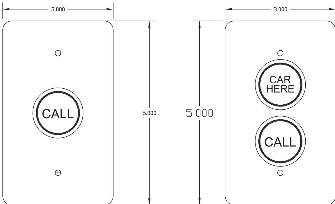
AUXILARY PANEL
