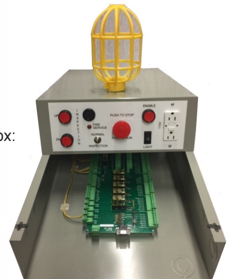
Car Top Box with Integrated Inspection Station
